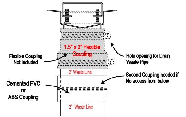
Drain Connection
